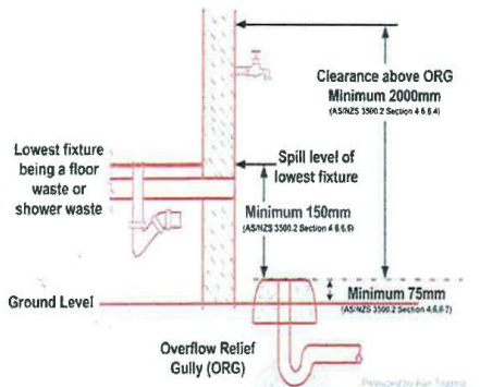
AS/NZS 3500.2:2003 - Overflow Relief Gully (ORG) requirements
