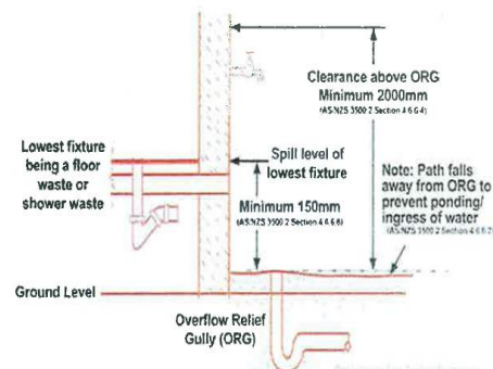
AS/NZS 3500.2:2003 - Overflow Relief Gully (ORG) requirements
