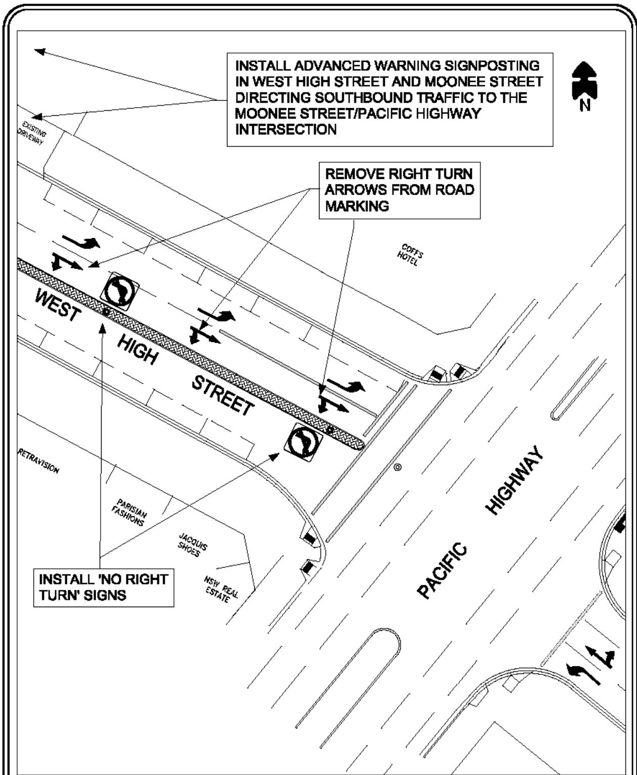
PLAN VIEW
