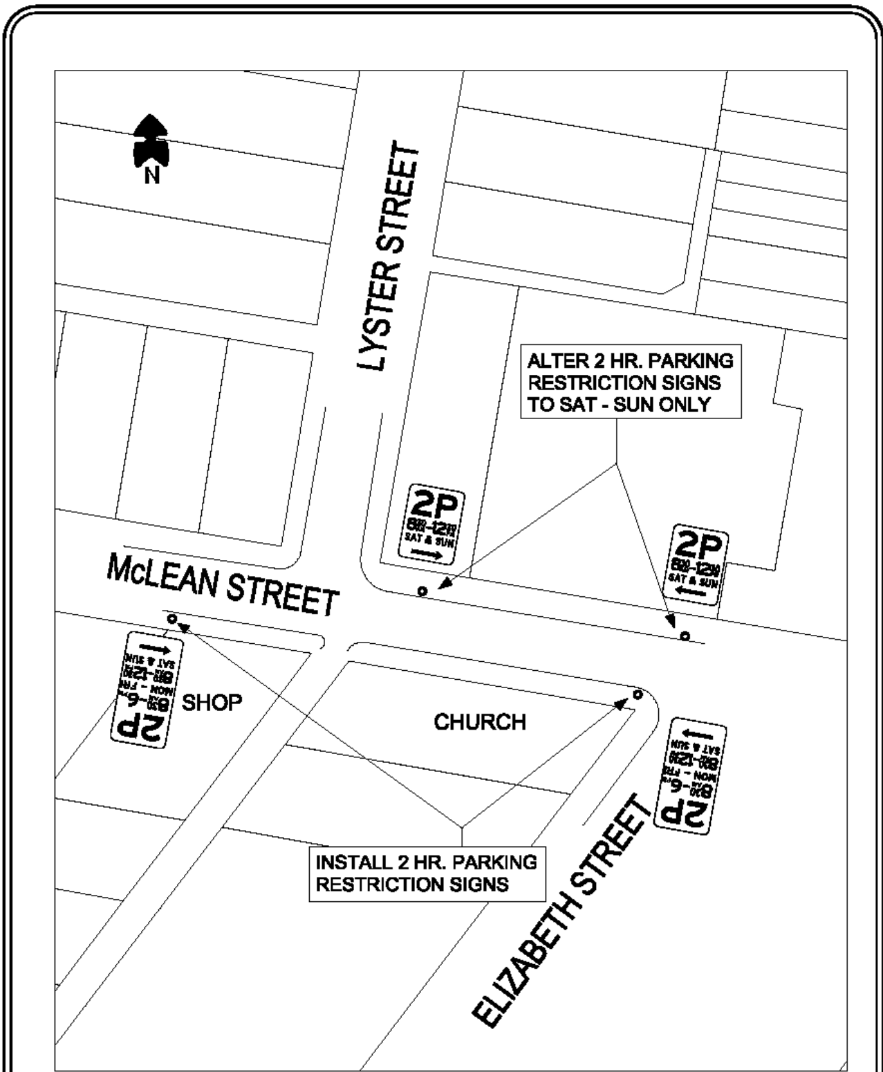
PLAN VIEW
